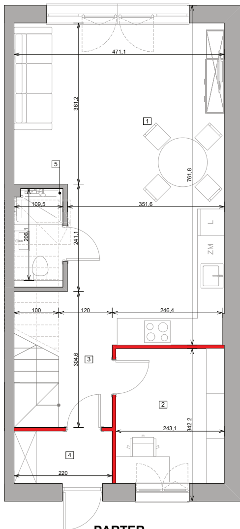
PARTER
